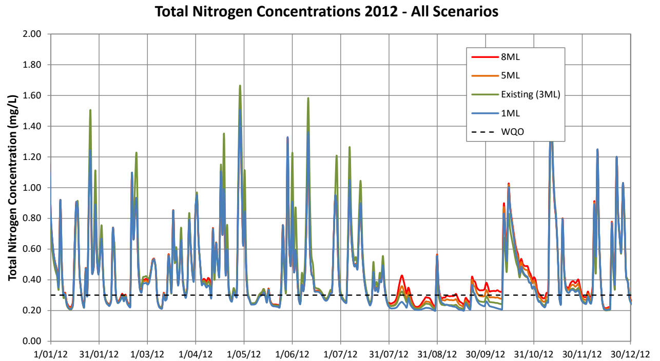
Figure 8-2 : Total Nitrogen Concentrations – All Scenarios
