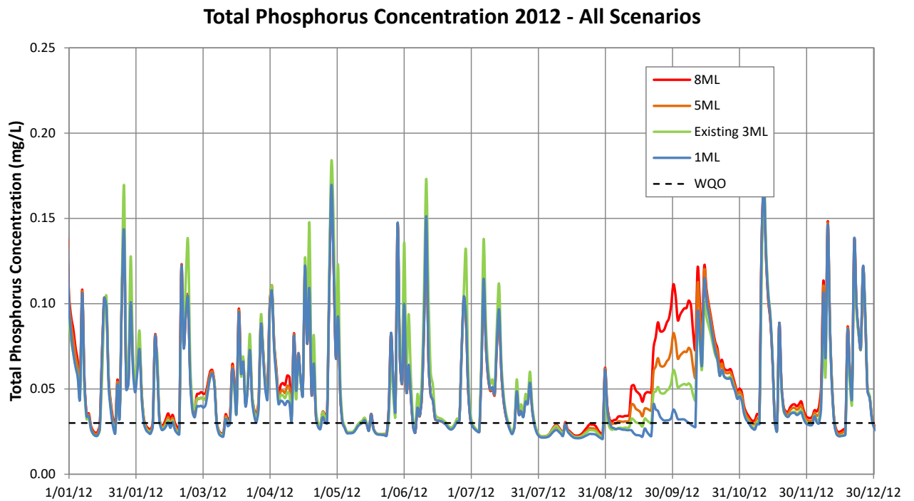
Figure 8-3 : Total Phosphorus Concentrations – All Scenarios
