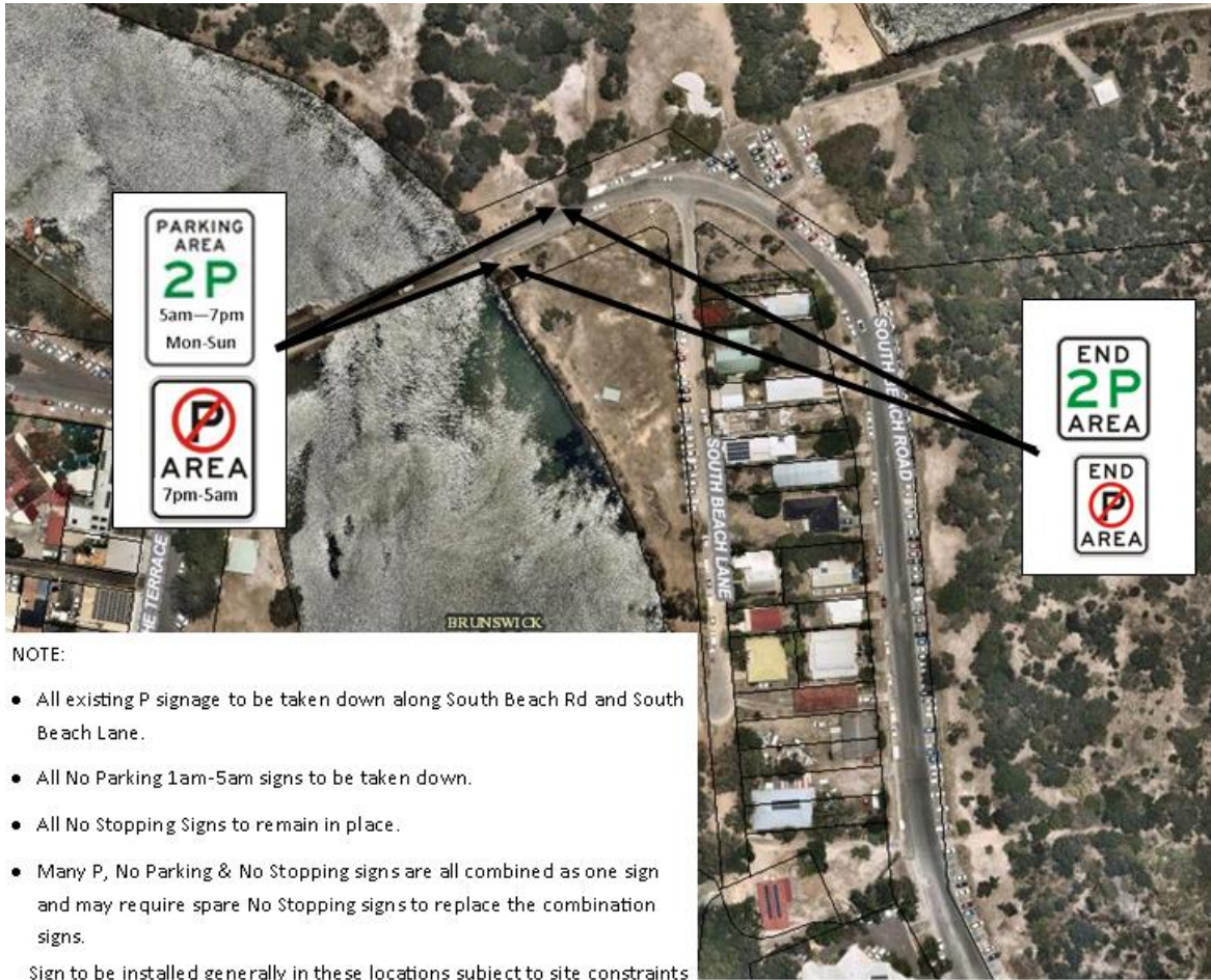
Figure 1. Signage plan
