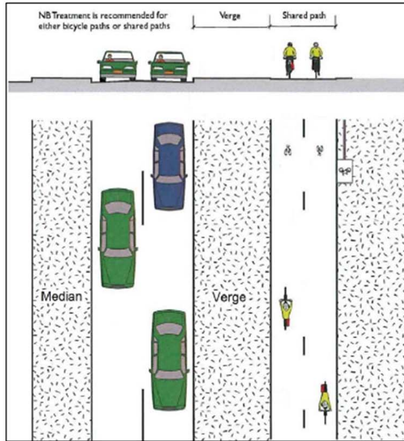
Figure 3.2: Bicycle path in a road reservation
