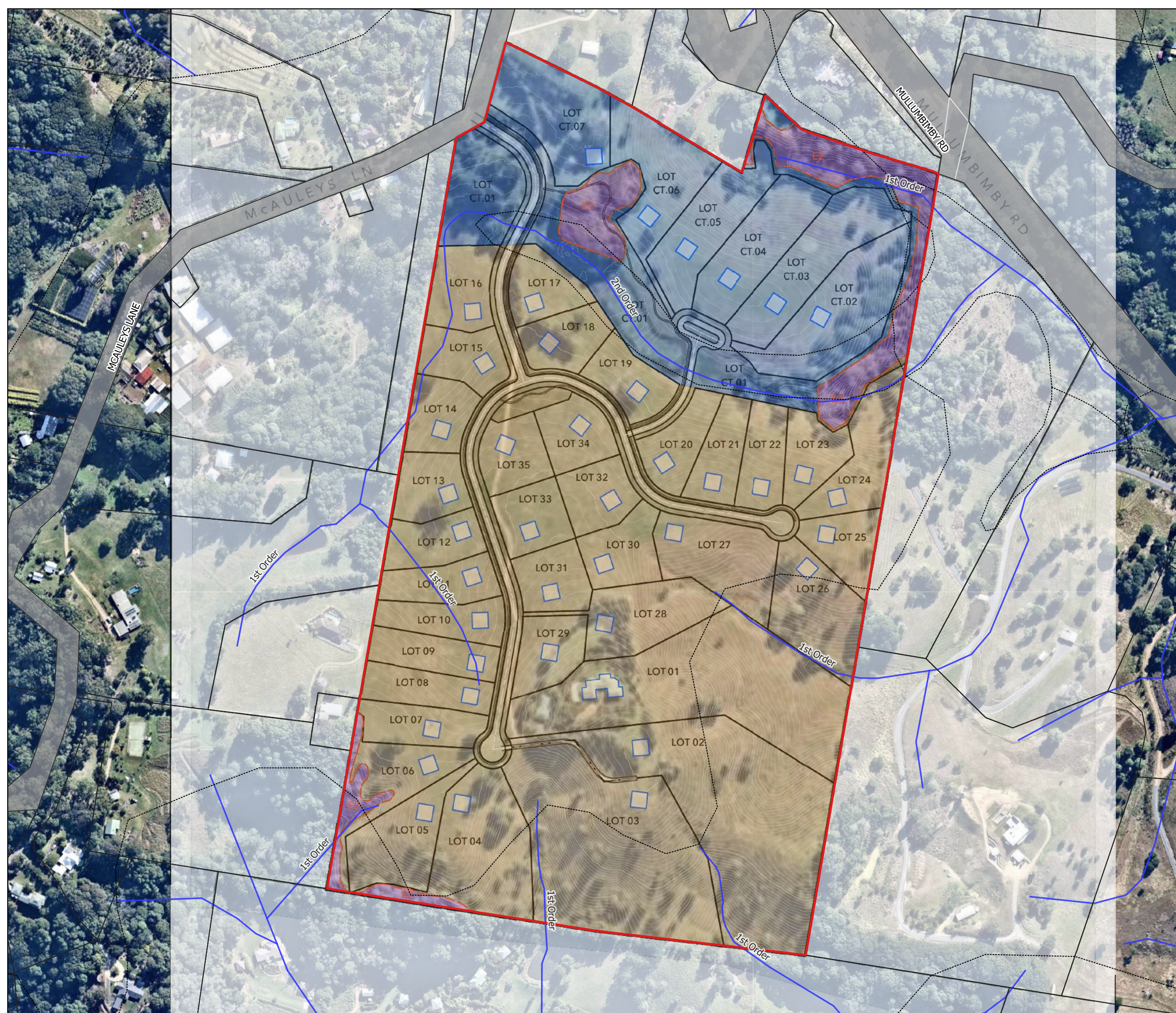
Figure 1.5: Concept site proposal – draft lot layout.
