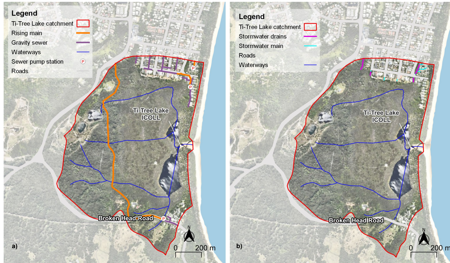
Figure 40: a) Ti-Tree Lake sewer and b) Ti-Tree Lake stormwater infrastructure
