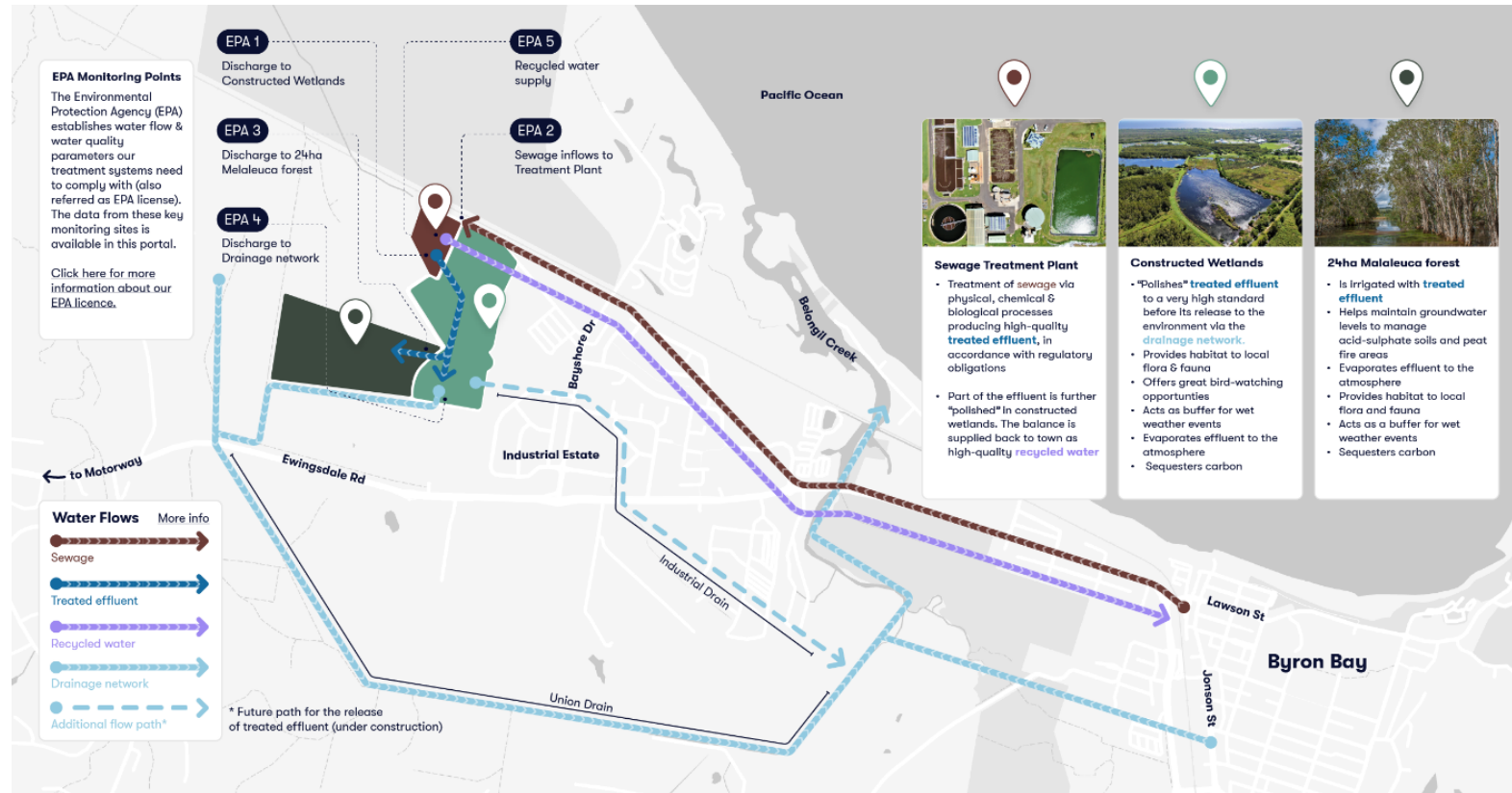
Figure 7: Byron Bay wastewater treatment process simplified infographic
