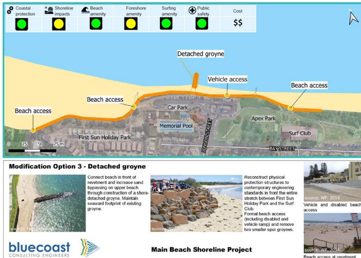
Figure 6: Option 3 – detached groyne.
