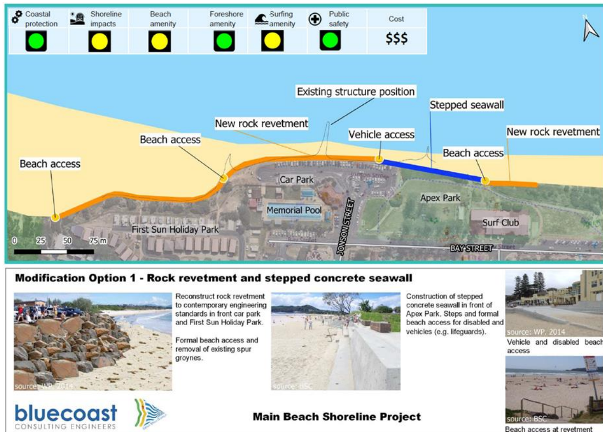
Figure 4: Modification option 1 – Rock revetment and stepped concrete seawall.
