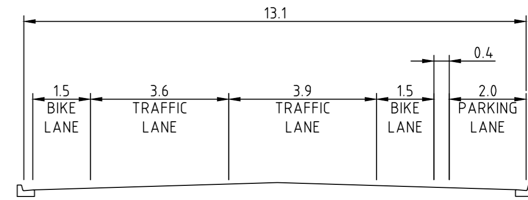
SECTION L-L
