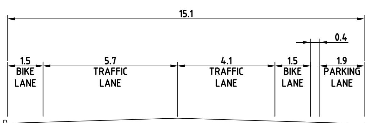
SECTION I-I
