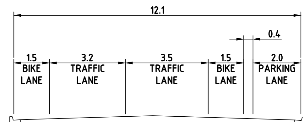
SECTION H-H
