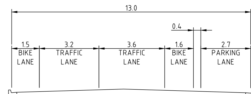
SECTION P-P
