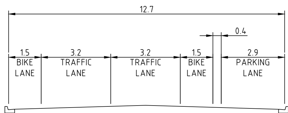
SECTION M-M
