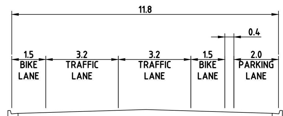
SECTION F-F
