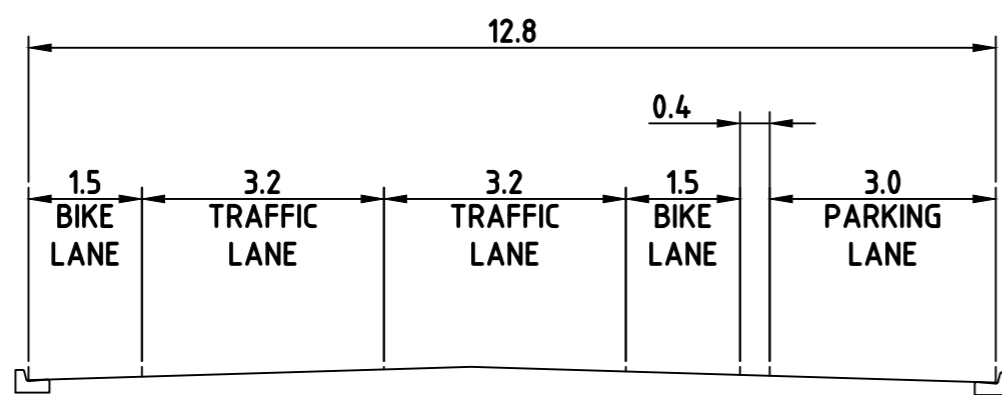
SECTION C-C
