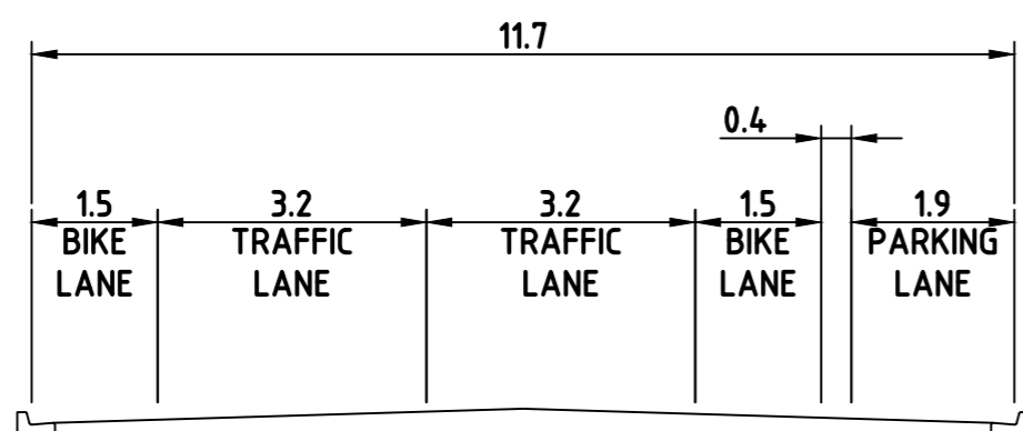
SECTION G-G
