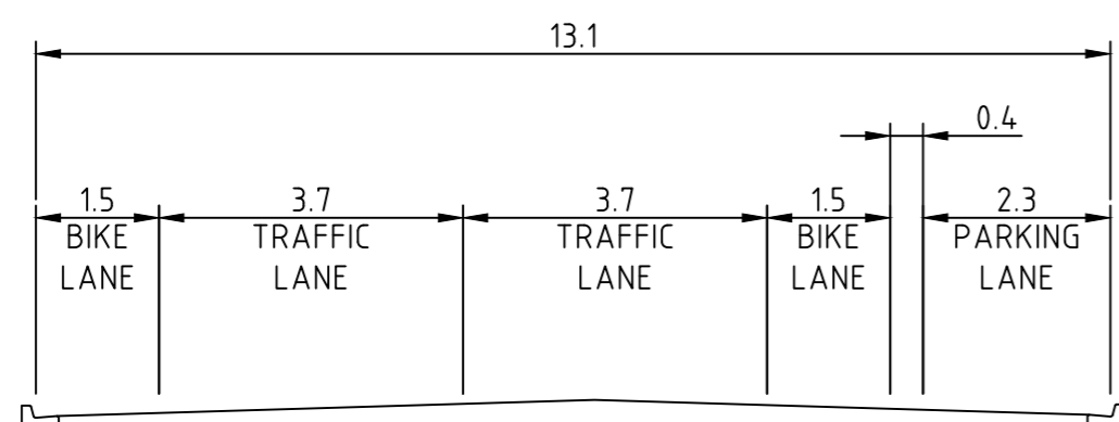
SECTION O-O
