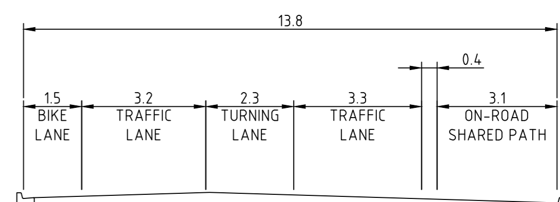
SECTION R-R
